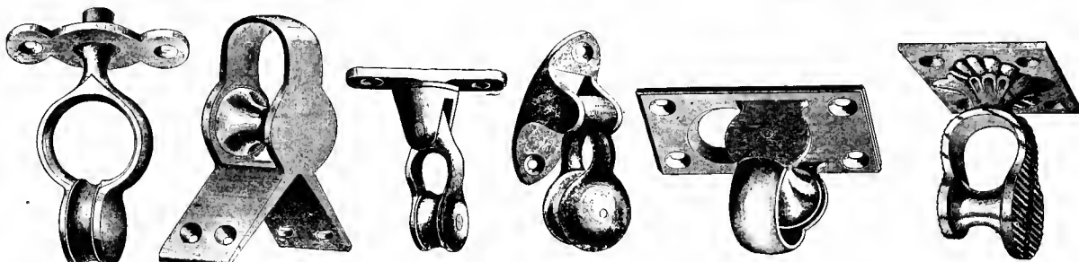
Fig. 2497. Fig. 2498. Fig. 2499. Fig. 2500. Fig. 2501. Fig. 2502. Overhead Guide with Pulley, Flange and Stem. Corner Guide with Pulley. Swing Guides with Pulleys. Angle Guides with Flanges and Pulleys.
